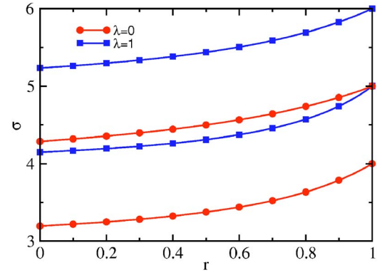
FIG. 2. (Color online) The exponent \sigma versus the restitution coefficient r for hard spheres ( \lambda=1 ) and Maxwell molecules ( \lambda=0 ). The top two curves are for d=3 and the bottom two curves are for d=2 .
