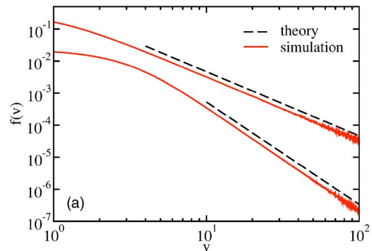
FIG. 3. (Color online) The velocity distribution for Maxwell molecules in one (top curves) and in two (bottom curves) dimensions.
