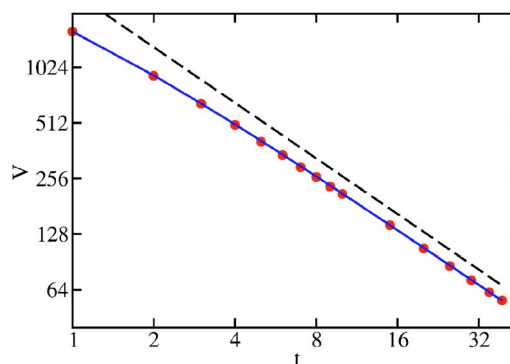
FIG. 8. (Color online) The cutoff velocity V(t) as a function of time t (circles). The solid line is a fit to Eq. (27). Also shown is a broken line with slope -1 .
