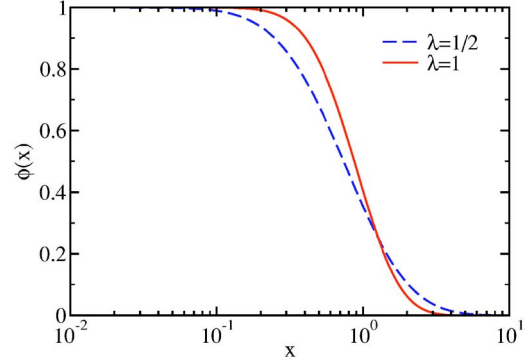
FIG. 5. (Color online) The scaling function \phi(x) versus x for \lambda=1/2 (dashed line) and 1 (solid line).
