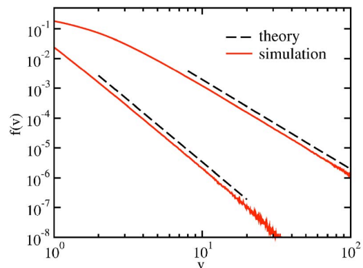
FIG. 4. (Color online) The velocity distribution for hard spheres in one (top curves) and in two (bottom curves) dimensions.
