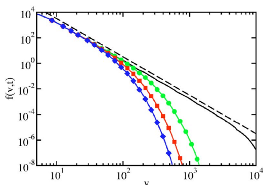
FIG. 6. (Color online) The velocity distribution f(v, t) versus v . Shown is the steady-state distribution before the injection is turned off (solid line) and at three consecutive and equally spaced later times (circles, squares, diamonds) during free cooling. Also shown for reference is a dashed line with slope -3 . The velocity is in arbitrary units.
