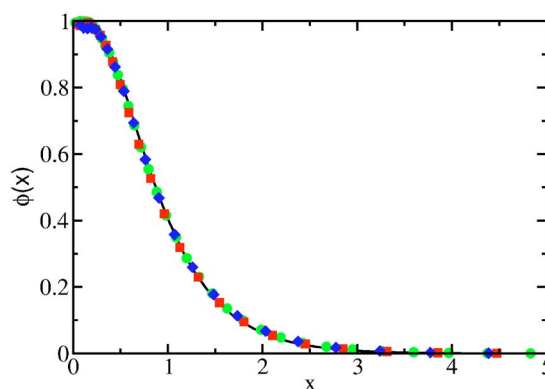
FIG. 7. (Color online) The scaling function underlying the velocity distribution. The velocity distributions in Fig. 6 were normalized by the stationary distribution as in Eq. (28). The solid line is the theoretical scaling function (35a) and (35b).
