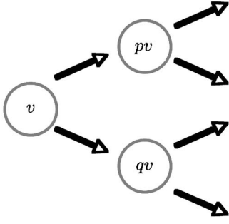
FIG. 1. The cascade process.
